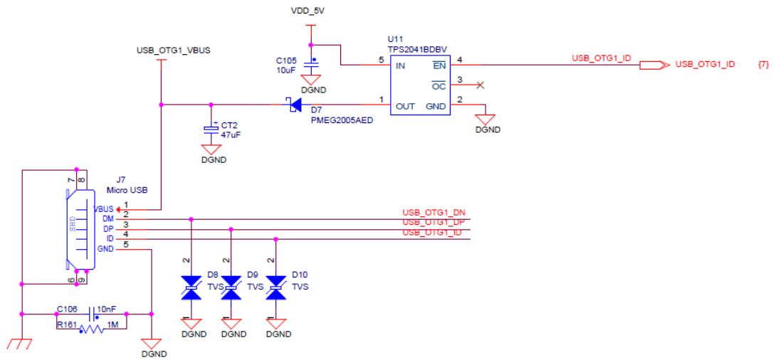
Figure 4-9 USB OTG
