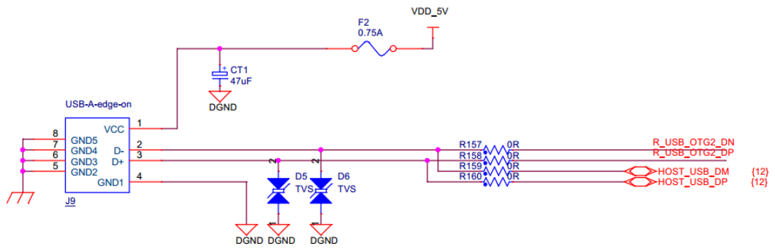
Figure 4-10 USB Host
