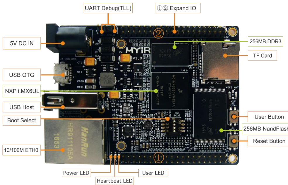
Figure 3-1 MYS-6ULX-IND Resources
