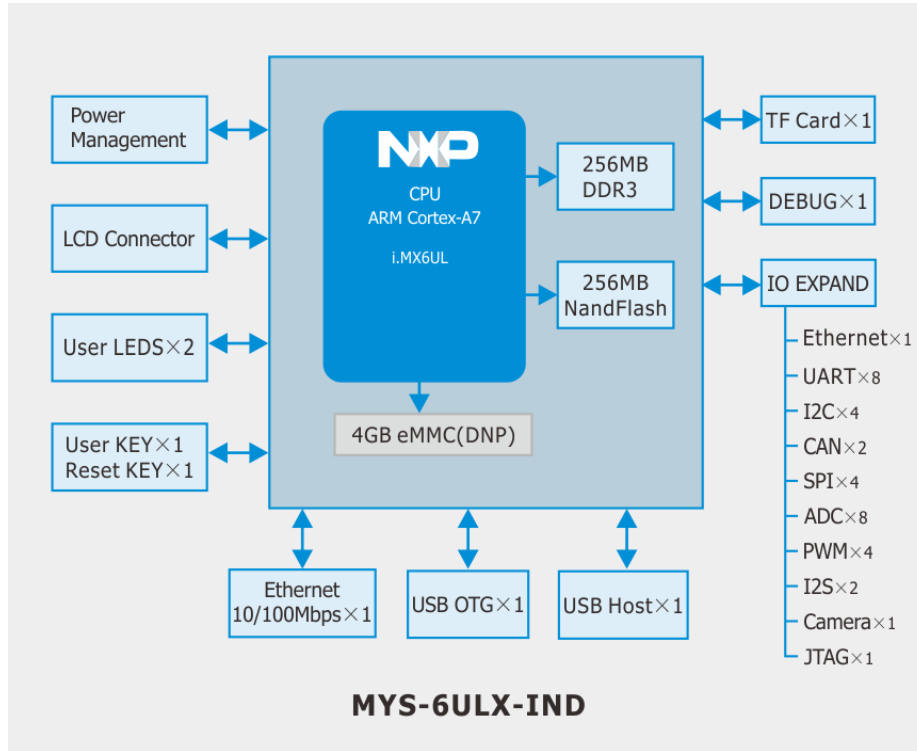
Figure 2-1 Function Block Diagram of MYS-6ULX-IND
