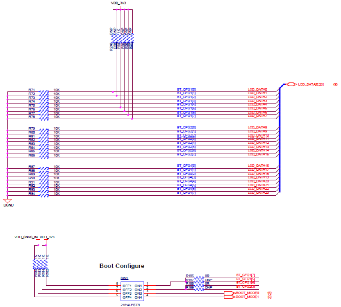
Figure 4-13 Boot Configure
