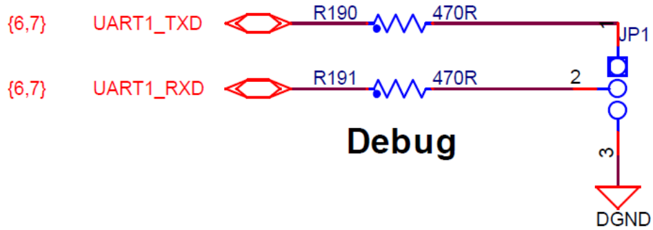
Figure 4-16 Debug UART
