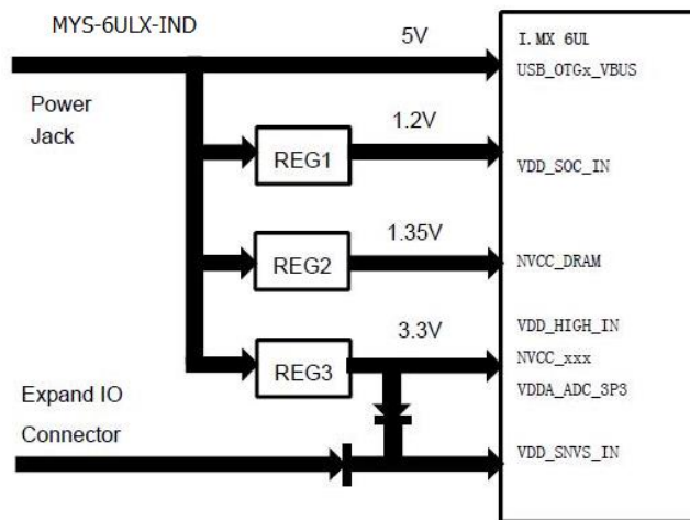
Figure 4-1 MYS-6ULX-IND Power Tree
