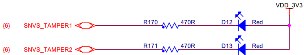
Figure 4-12 User LEDs
