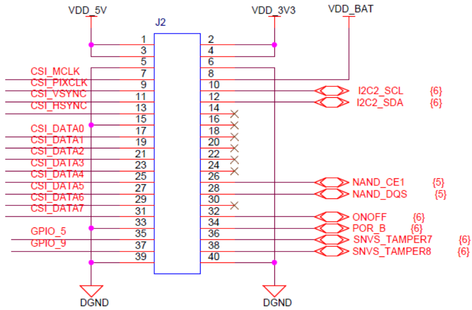
Figure 4-14 Expansion Interface (J2)
