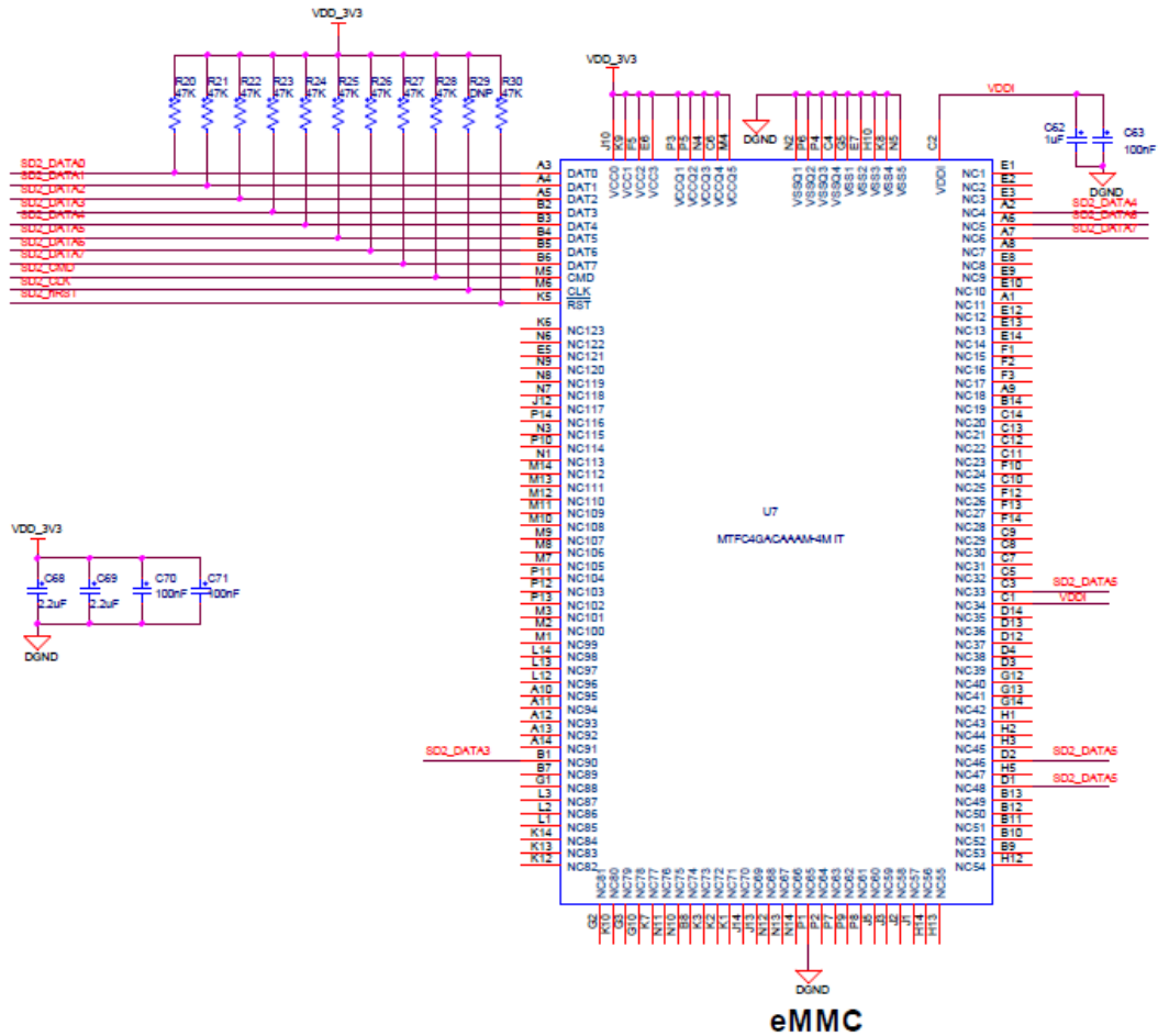
Figure 4-4 eMMC Memory
